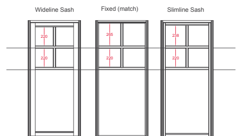
Illustration of a 1372mm high awning window.
